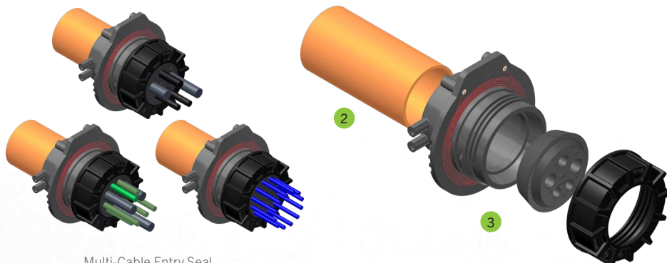
Multi-Cable Entry Seal Compression Disc Options
